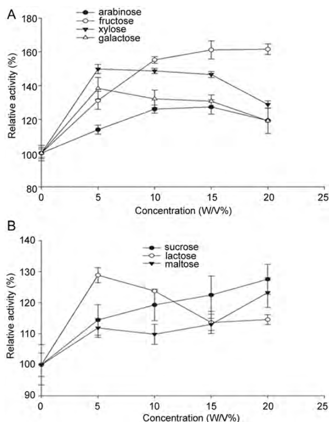
Figure 6 Effects of mono- and disaccharides on p -NPG hydrolysis by Unbgl1A. (A) Effect of monosaccharide (L-arabinose, D-fructose, xylose, and D-galactose) on p -NPG hydrolysis by Unbgl1A. (B) Effect of disaccharides (sucrose, lactose, and maltose) on p -NPG hydrolysis by Unbgl1A. The activity measured without any additive (as control) was considered to be 100%.
