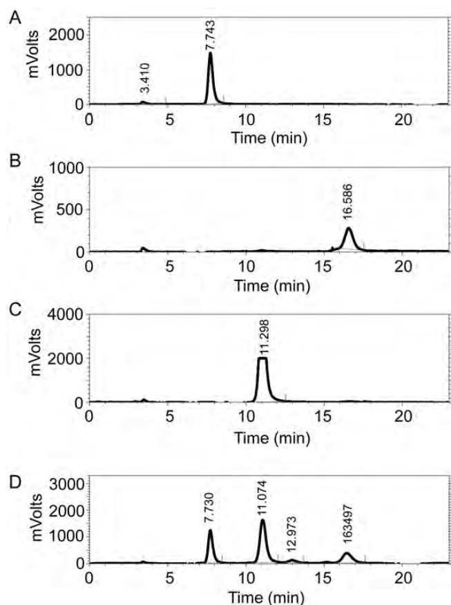
Figure 9 HPLC analysis of the hydrolysis products of cellobiose by Unbgl1A (A) Standard glucose. (B) Standard cellotriose. (C) Hydrolysis products of control. (D) Hydrolysis products of cellobiose by Unbgl1A.
