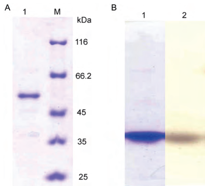
Figure 3 PAGE analysis of recombinant Unbgl1A (A) Purified recombinant Unbgl1A was detected by SDS-PAGE. Lane M: protein molecular weight marker. Lane 1: purified Unbgl1A. Recombinant protein was purified with Ni-NTA chromatography. (B) Purified recombinant Unbgl1A was analyzed by non-denaturing PAGE and zymogram. Lane 1: recombinant Unbgl1A stained using Coomassie Brilliant Blue R250. Lane 2: recombinant Unbgl1A incubated with 0.1% esculin hydrate and 0.25% ferric ammonium citrate.
