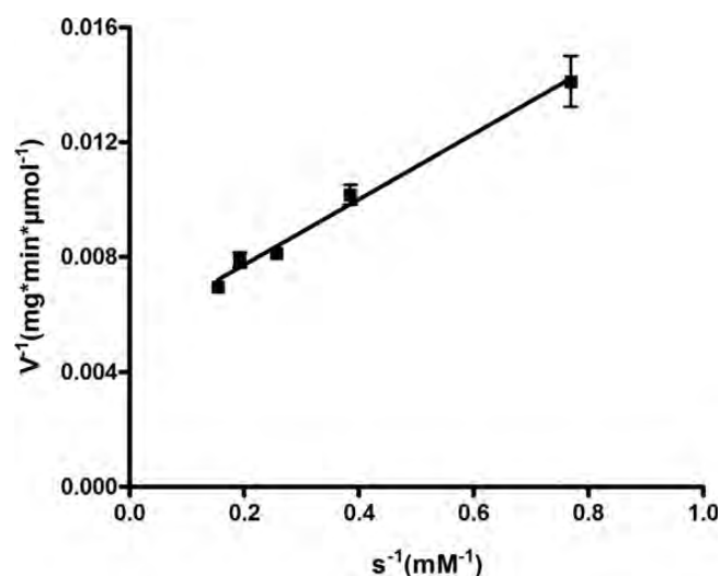
Figure 7 Lineweaver–Burk plot of Unbgl1A. Unbgl1A had a K_m value of 2.09 \pm 0.31 mM and a V_{max} value of 183.9 \pm 9.61 \mu\text{mol min}^{-1} \text{mg}^{-1} in the presence of p -NPG.
