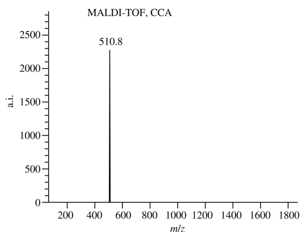
Fig. 3 MALDI-TOF mass spectrum of OEP3121
