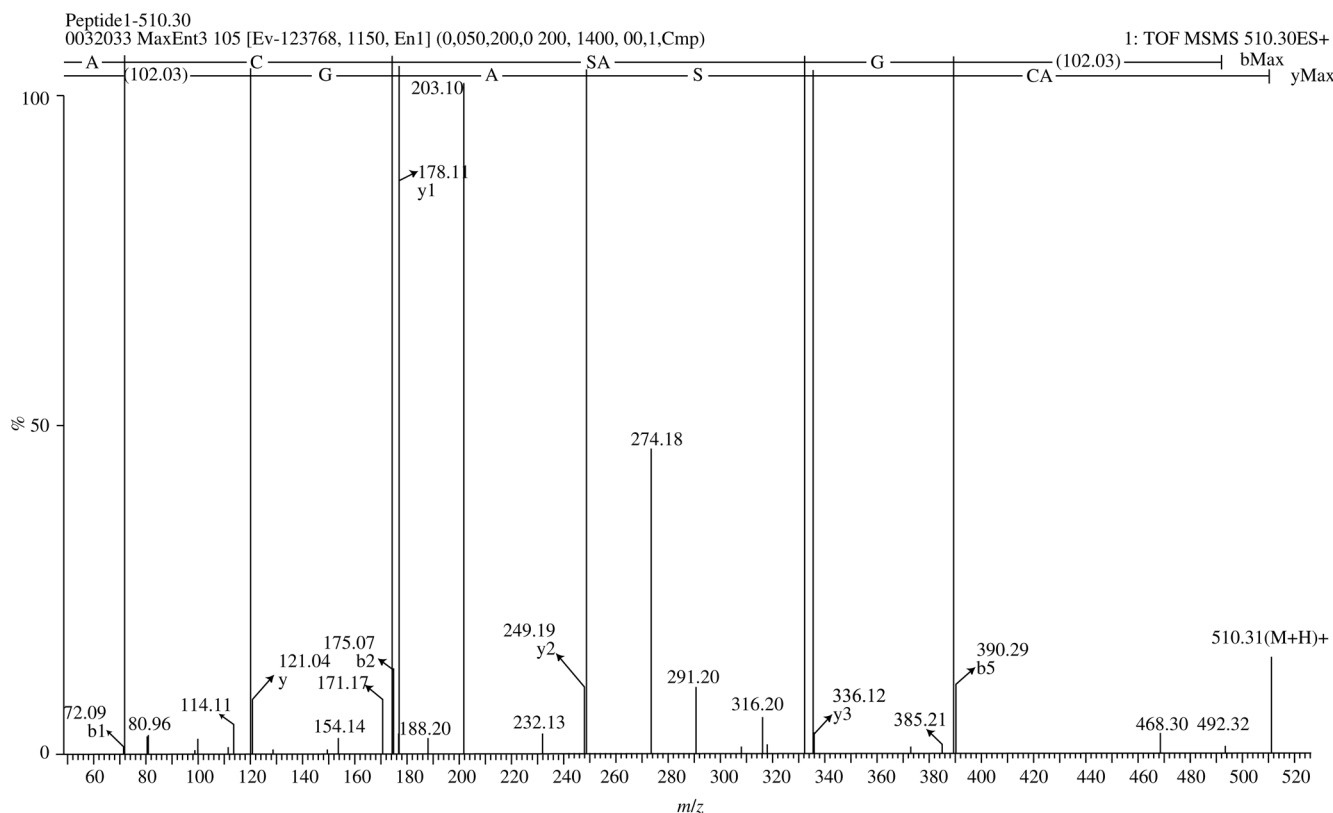
Fig. 4 Amino acid sequencing of OEP3121 by MS-MS
