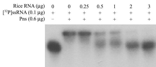
Fig. 6 Competition assays of total rice RNA with ^{32} P-labeled RRSV S9 ssRNA for binding to Pns6
