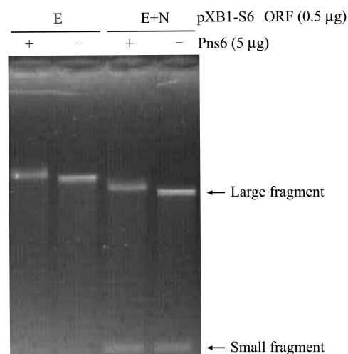
Fig. 3 Binding of Pns6 with different kinds of nucleic acids in gel mobility shift assay
