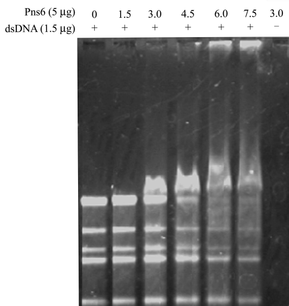
Fig. 3 Binding of Pns6 with different kinds of nucleic acids in gel mobility shift assay
