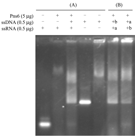
Fig. 5 Competition (A) and displacement (B) assays between ssRNA and ssDNA for binding to Pns6 a, first added; b, second added.
