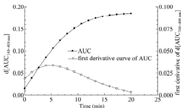
Fig. 2 Time progress of p -nitrophenyl \beta -D-cellobioside (200 \mu M) hydrolyzed by 1,4- \beta -D-glucan cellobiohydrolase I (1.0 \mu M) at 50 °C in acetate buffer
