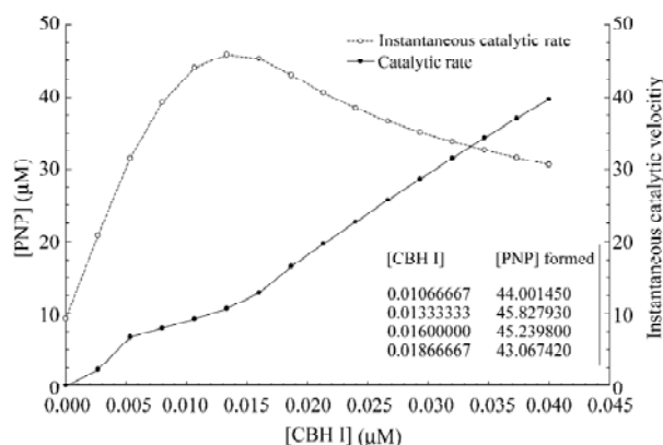
Fig. 4 Companson of catalytic cure and its instaneous rate cure of PNPC (100 \mu\text{M} ) hydrolyzed by different concentration of CBH I
